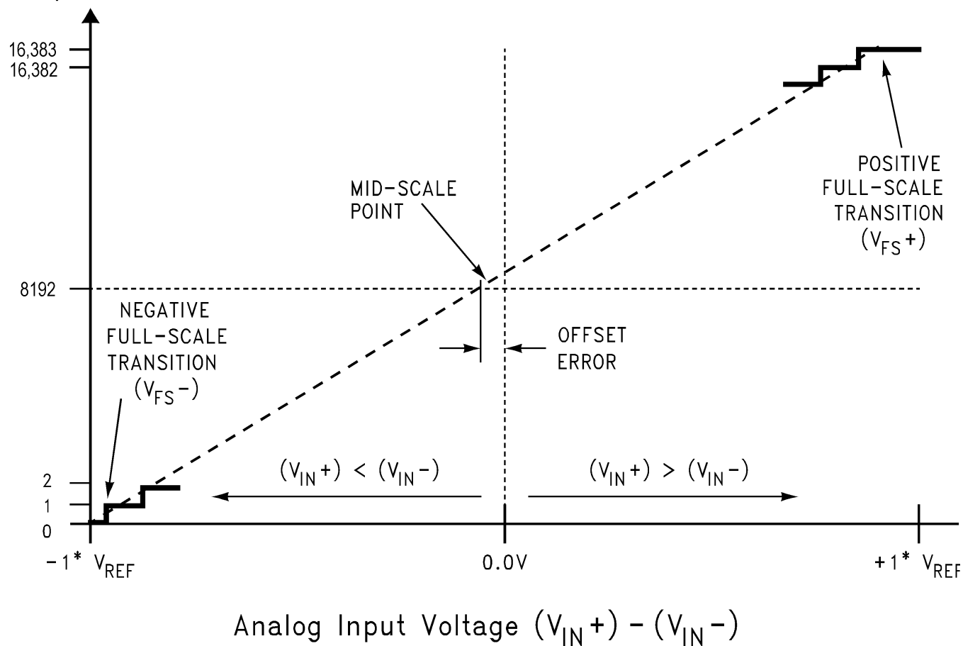
Figure 3. Transfer Characteristic
