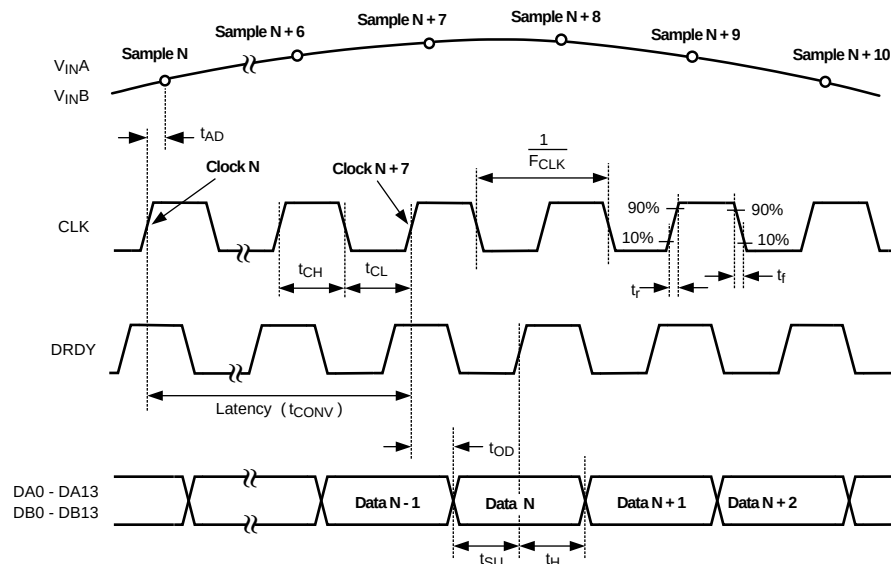
Figure 2. Output Timing
